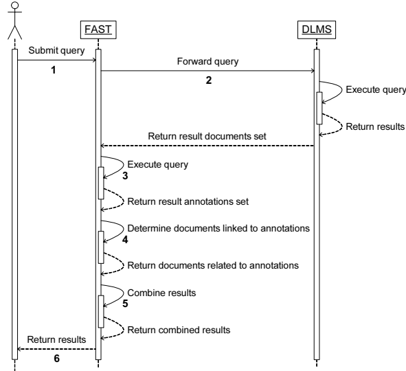
Fig. 2. UML sequence diagram of the search strategy for searching documents by exploiting annotations (from [3])
