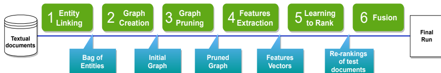
Fig. 1: Representation of the main phases composing the proposed solution. Green rectangles show the six phases, while the blue ones show the output of each phase.
