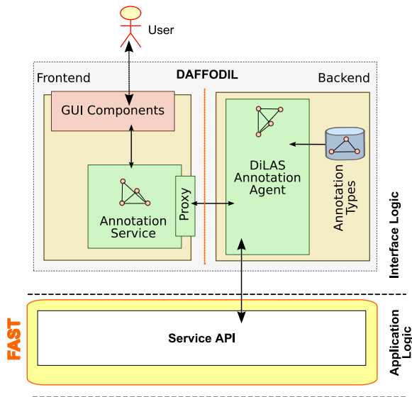
Figure 4: DAFFODIL/DiLAS Architecture
