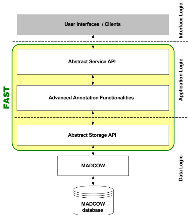
Figure 2: DiLAS Architecture
