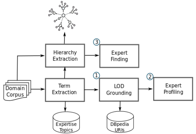
Fig. 9 Data flow of the semantic enrichment approach
