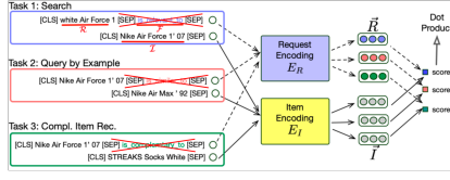
(a) Removing task label from UIA architecture.
