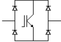
Fig. 9 – Bi-directional switch used in the prototype.
