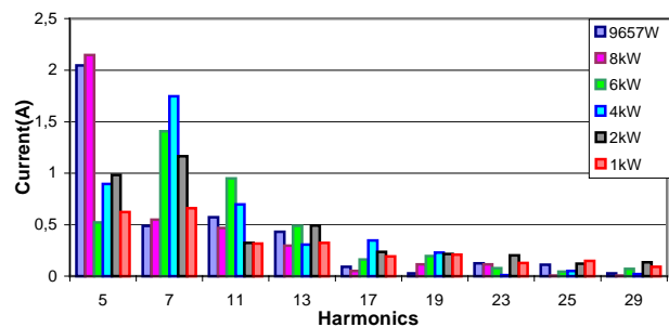
Fig. 8 – Input current harmonic amplitudes at different power levels
