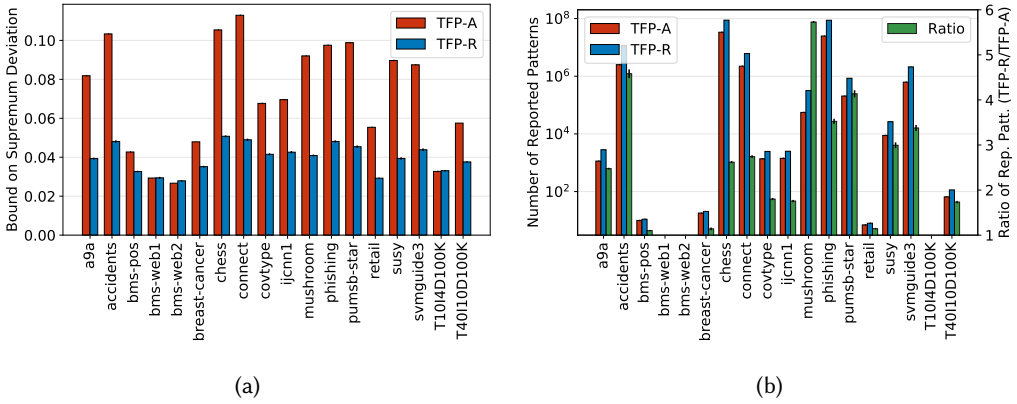
Fig. 5. (a) Bounds on the Supremum Deviation obtained by TFP-R and TFP-A for \theta = 0.05 . (b) Number of reported patterns (left y -axis) and ratios (right y -axis) by TFP-R and TFP-A.
