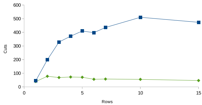
Figure 4: Number of cuts generated ( \square ) and tight at the end ( \diamond ), on 62 instances
