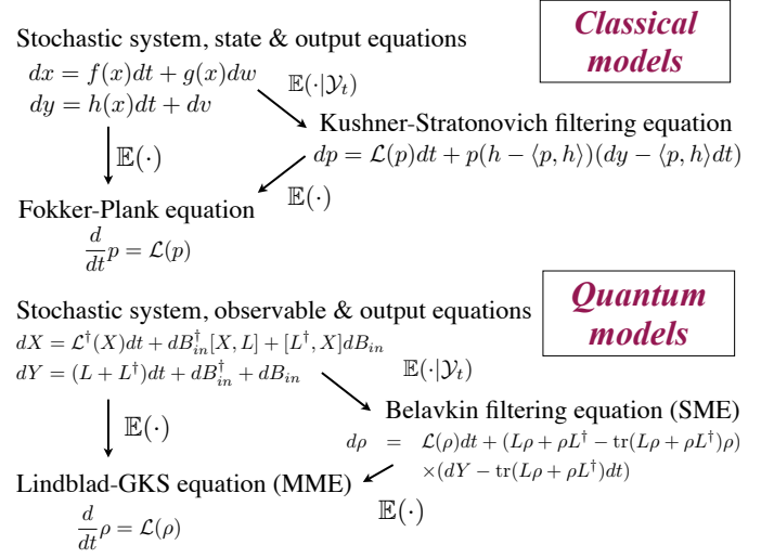
Fig. 1. A parallel between the models of classical and quantum stochastic dynamics, and the role of expectations. Adapted from [84].
