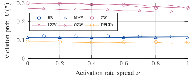
Fig. 8: V(5) as a function of \nu with \rho = 0.5 .
