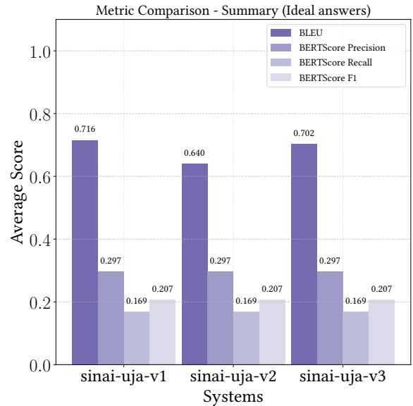
Figure 7: Evaluation for Summary answers.
