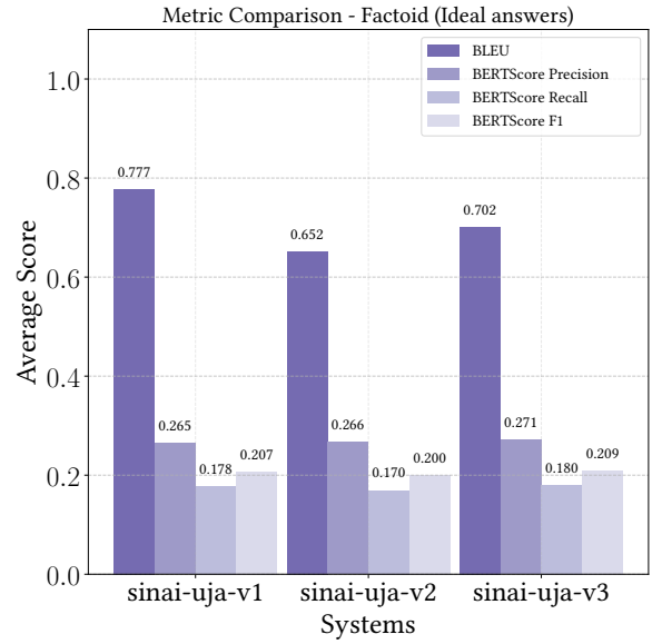
Figure 5: Evaluation for ideal Factoid answers.
