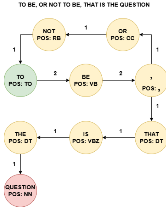
Figure 1: Word Adjacency Network example
