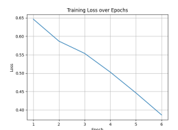
(b) ModernBERT-large
