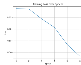
(h) XLM-RoBERTa-large
