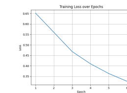
(h) XLM-RoBERTa-large
