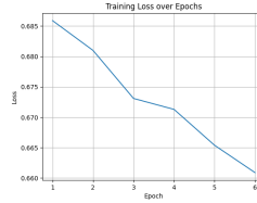
(c) BERT-base
