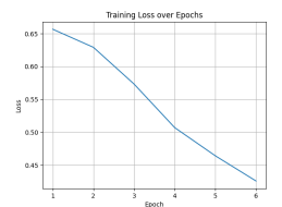
(f) RoBERTa-large
