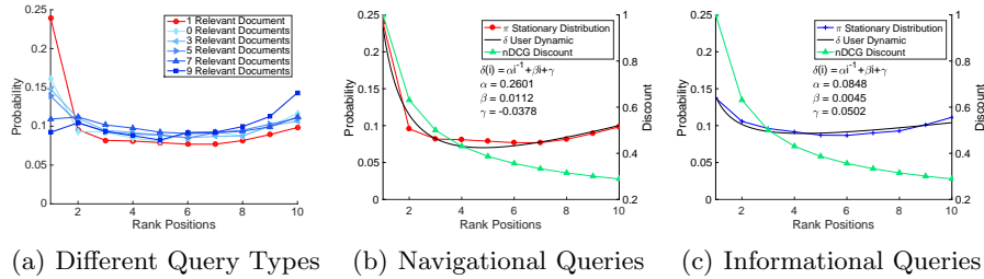
Fig. 1. Stationary distributions for queries retrieving different numbers of relevant documents (a); and stationary distribution with its fitted curve and DCG discount for navigational (b), and informational queries (c).
